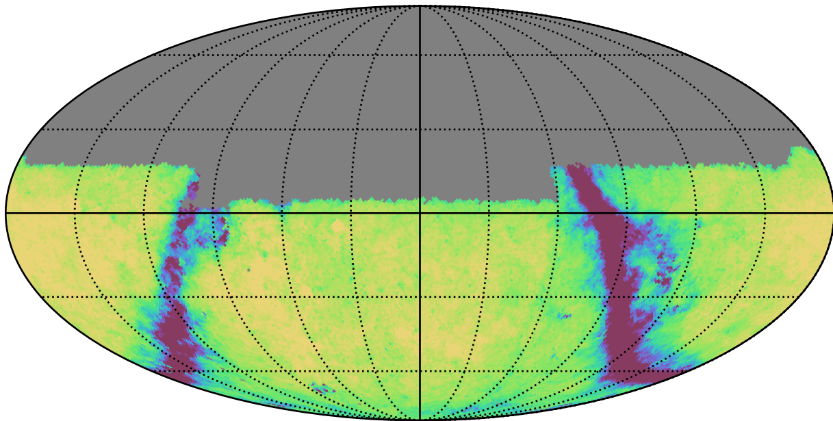
baseline_v3.2_10yrs Yr 1 u band: Exgal_CoaddM5
