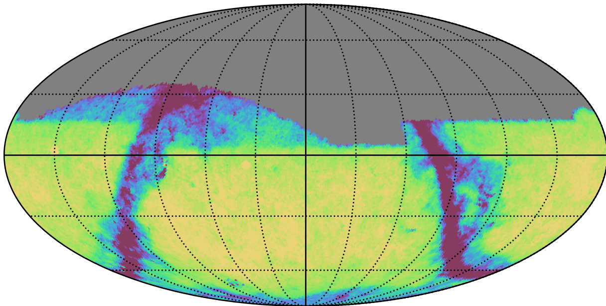
baseline_v3.2_10yrs Yr 1 i band: Exgal_CoaddM5
