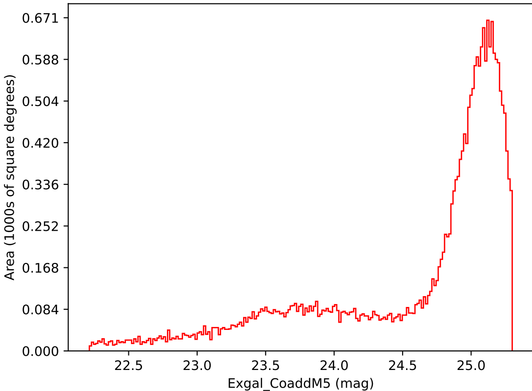
baseline_v3.2_10yrs Yr 1 i band: Exgal_CoaddM5
