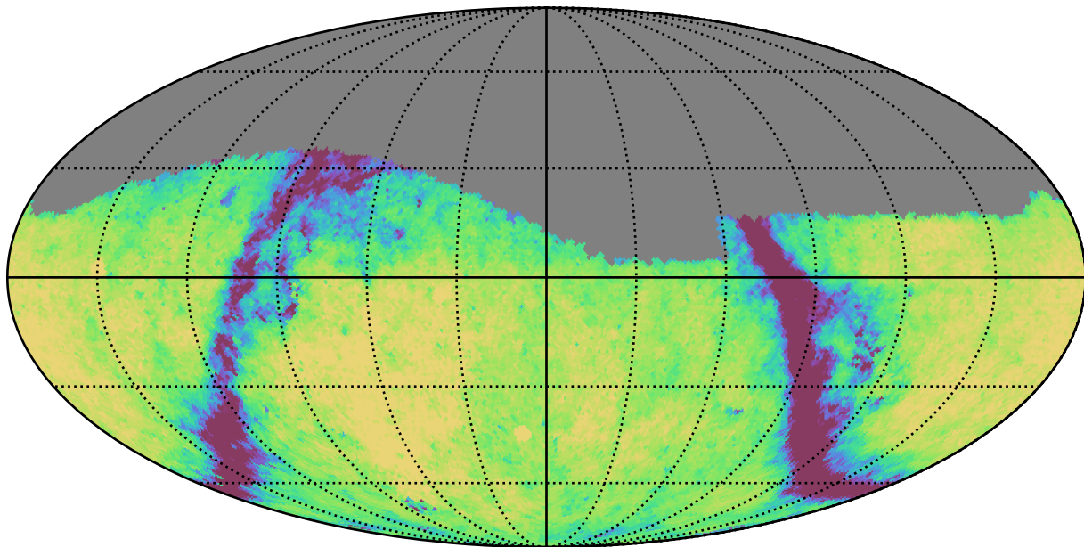
baseline_v3.2_10yrs Yr 1 g band: Exgal_CoaddM5
