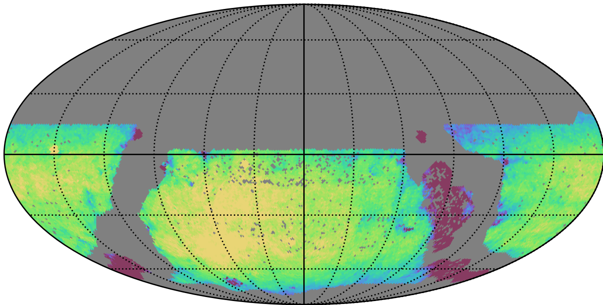
baseline_v3.2_10yrs WFD z band: Exgal_CoaddM5
