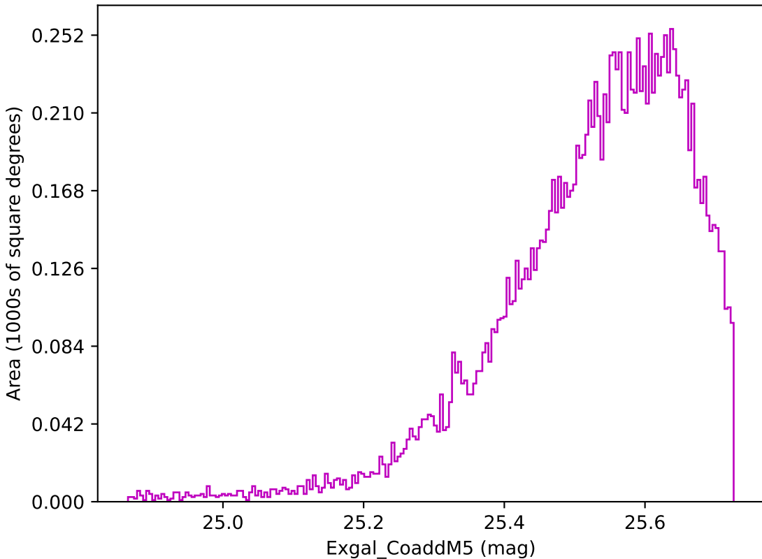
baseline_v3.2_10yrs WFD z band: Exgal_CoaddM5
