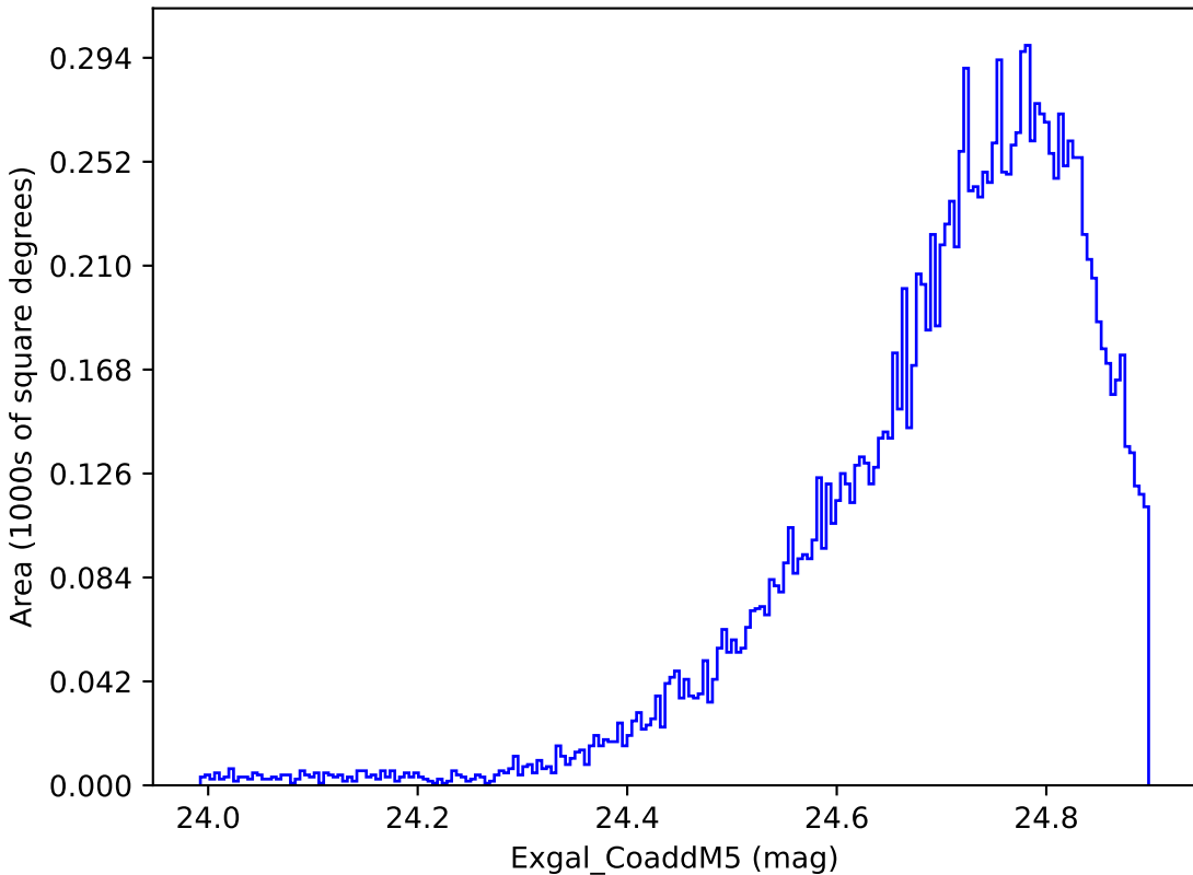
baseline_v3.2_10yrs WFD y band: Exgal_CoaddM5
