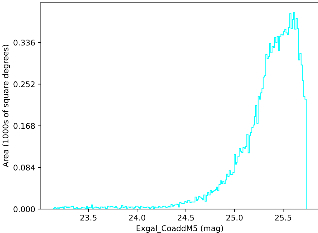
baseline_v3.2_10yrs WFD u band: Exgal_CoaddM5
