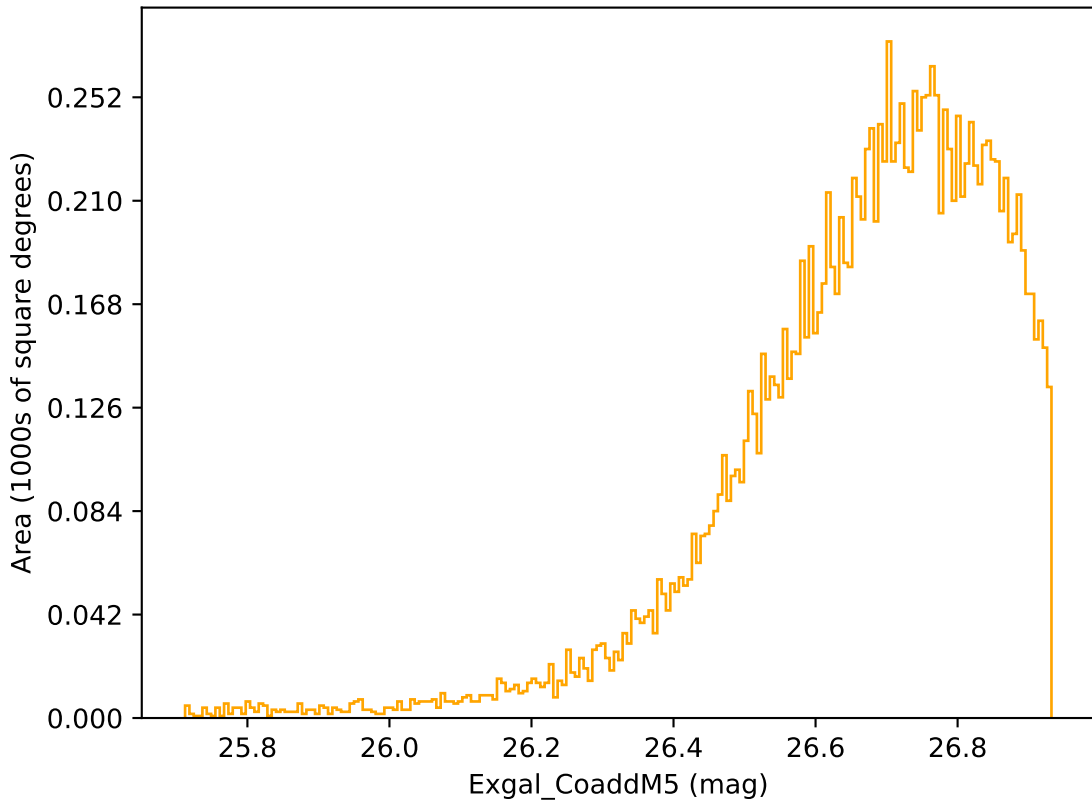
baseline_v3.2_10yrs WFD r band: Exgal_CoaddM5
