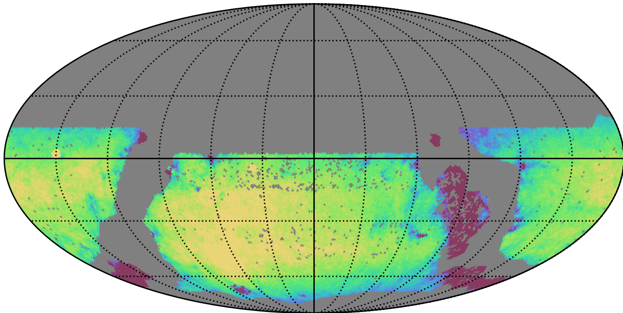
baseline_v3.2_10yrs WFD i band: Exgal_CoaddM5
