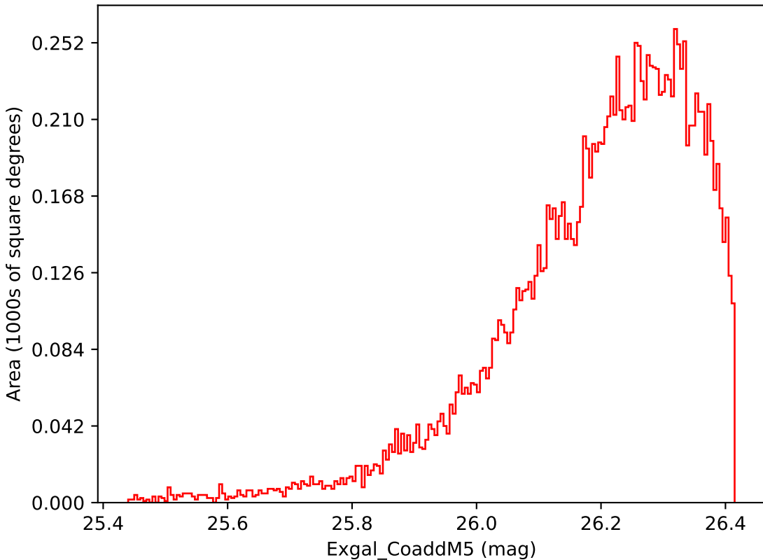
baseline_v3.2_10yrs WFD i band: Exgal_CoaddM5
