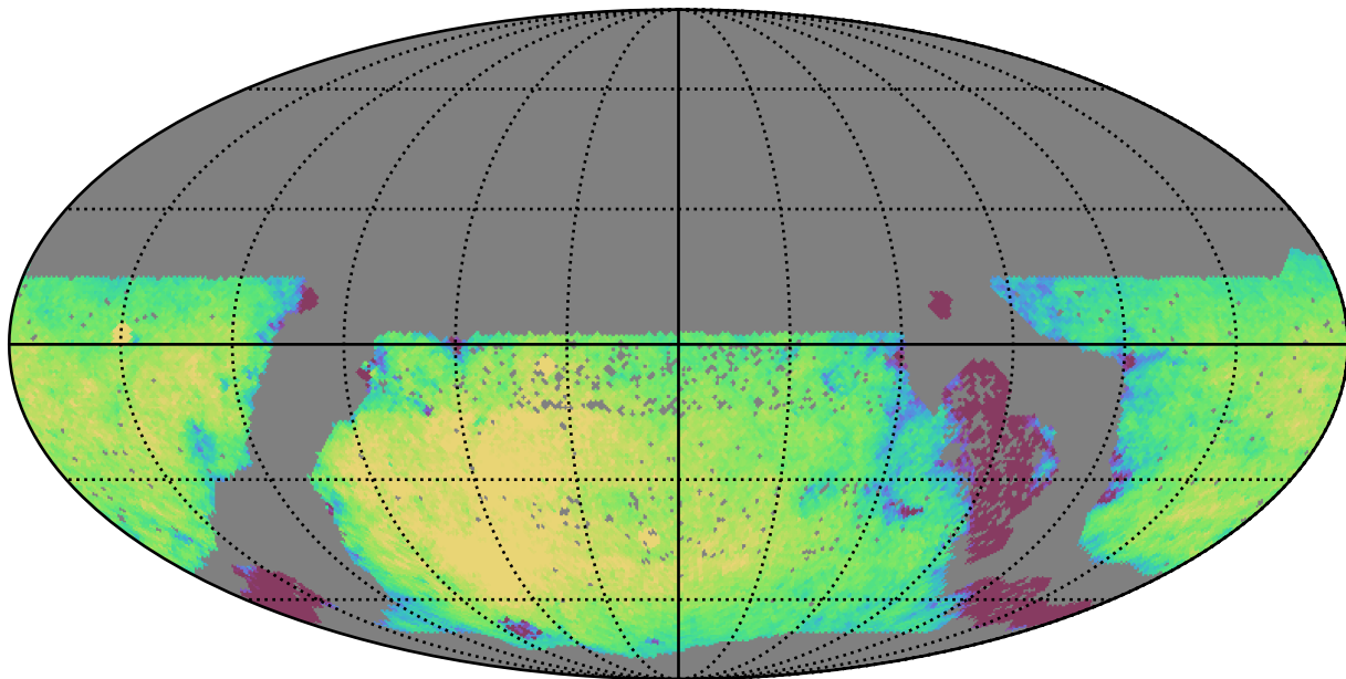
baseline_v3.2_10yrs WFD g band: Exgal_CoaddM5
