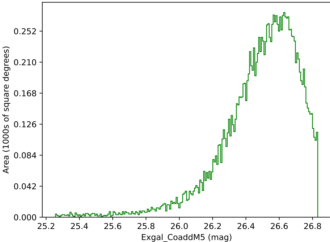
baseline_v3.2_10yrs WFD g band: Exgal_CoaddM5
