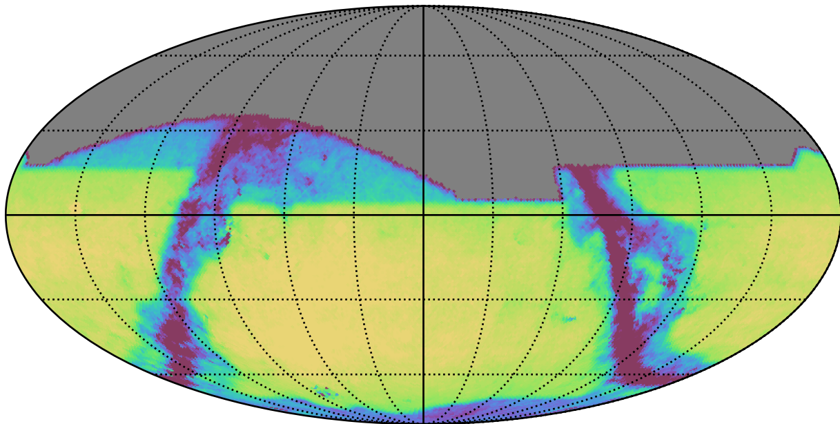
baseline_v3.2_10yrs All sky z band: Exgal_CoaddM5
