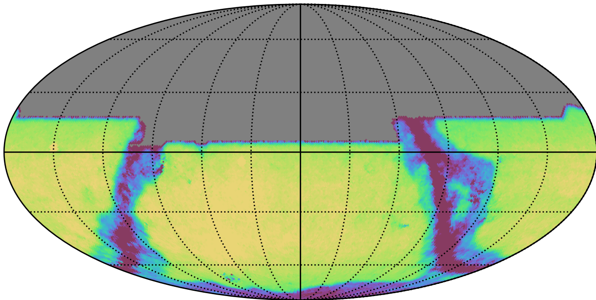
baseline_v3.2_10yrs All sky y band: Exgal_CoaddM5
