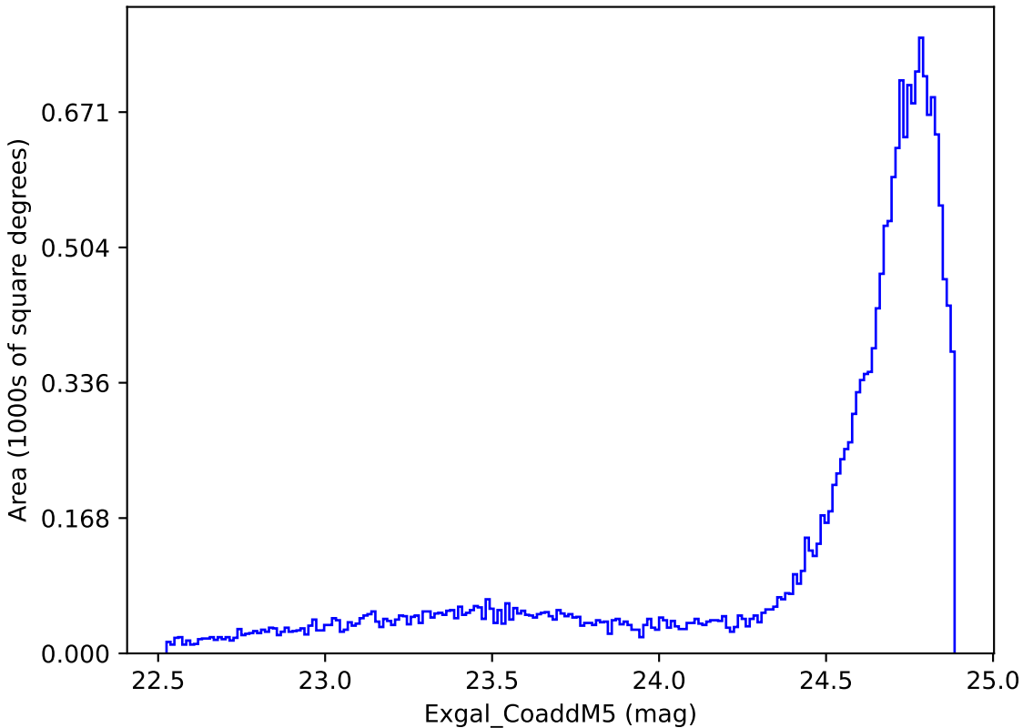
baseline_v3.2_10yrs All sky y band: Exgal_CoaddM5
