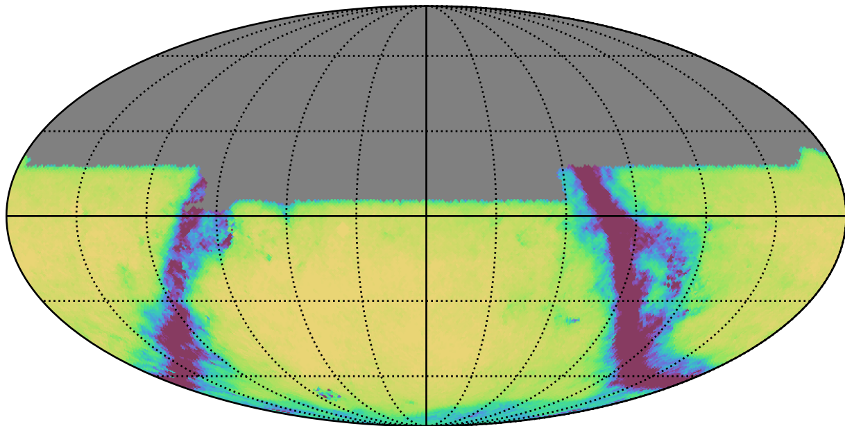
baseline_v3.2_10yrs All sky u band: Exgal_CoaddM5
