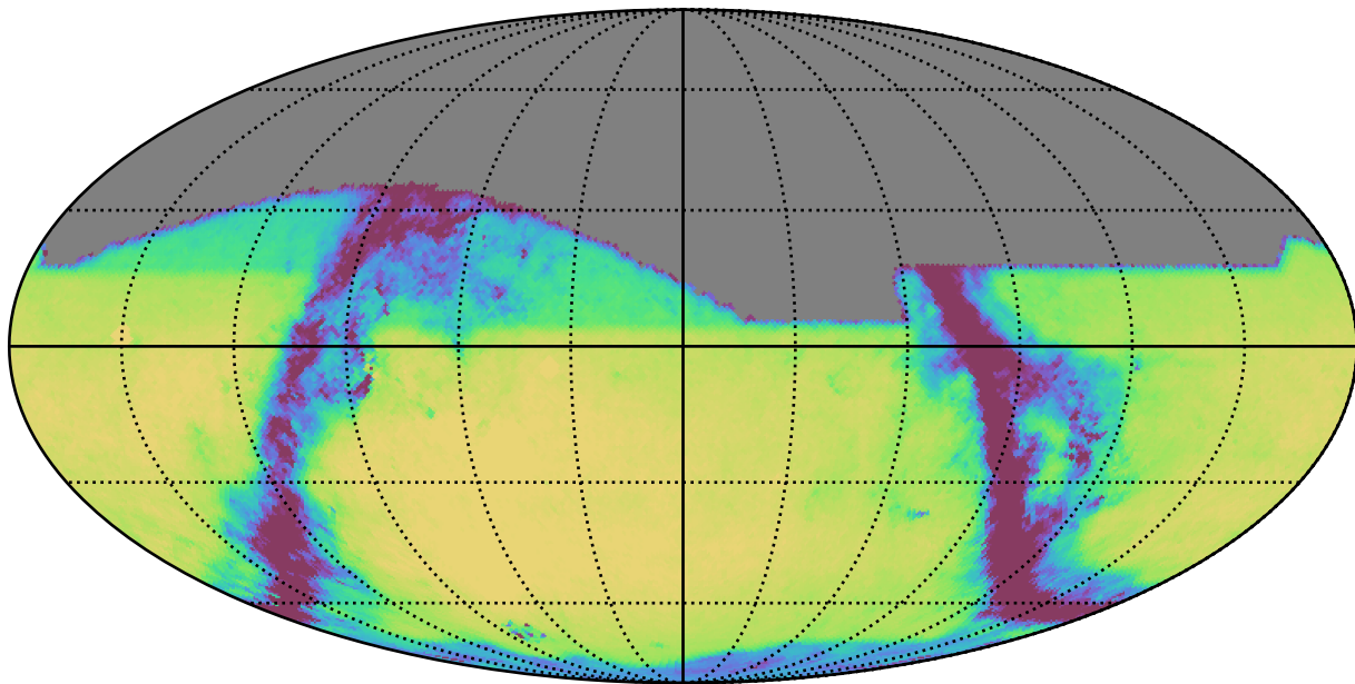
baseline_v3.2_10yrs All sky r band: Exgal_CoaddM5
