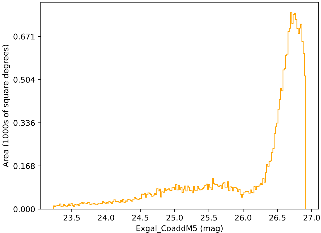
baseline_v3.2_10yrs All sky r band: Exgal_CoaddM5
