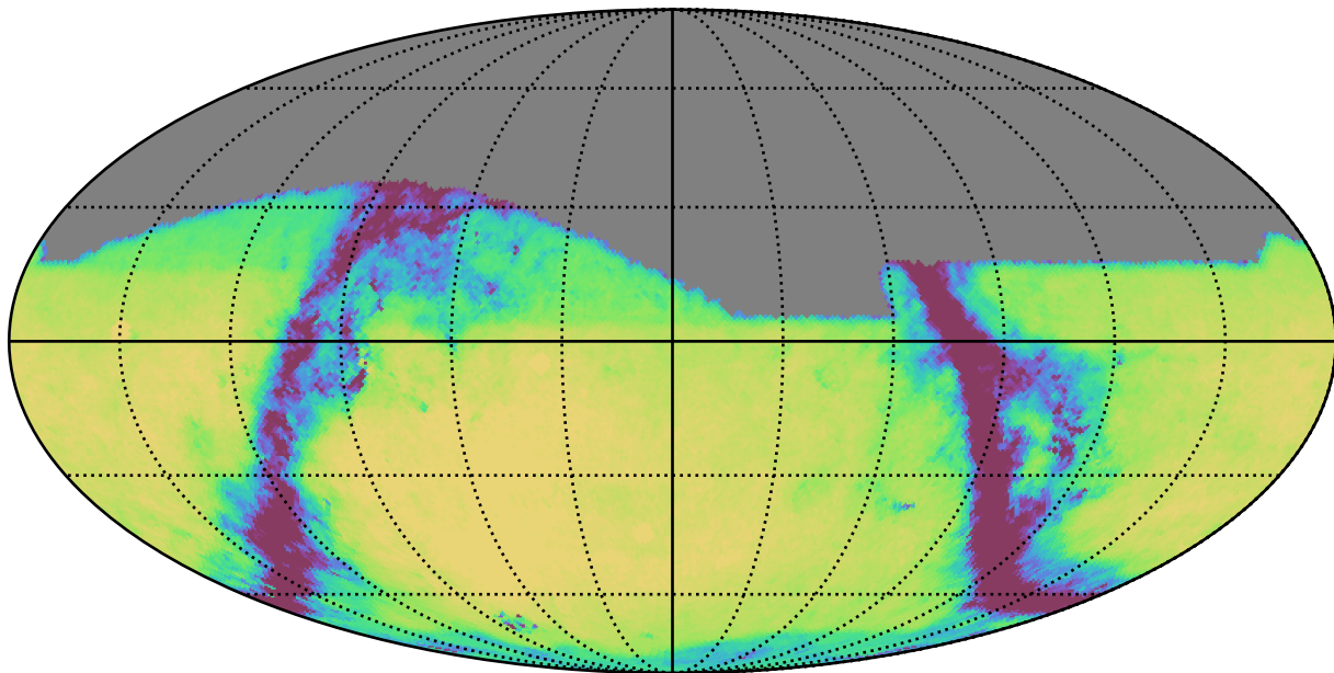
baseline_v3.2_10yrs All sky g band: Exgal_CoaddM5
