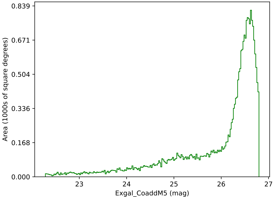
baseline_v3.2_10yrs All sky g band: Exgal_CoaddM5
