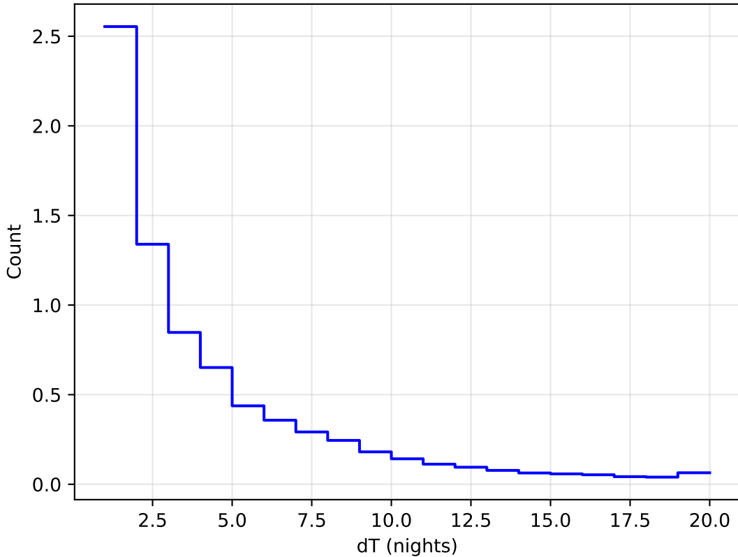
baseline_v3.2_10yrs WFD all bands: DeltaNight Histogram 1e6
