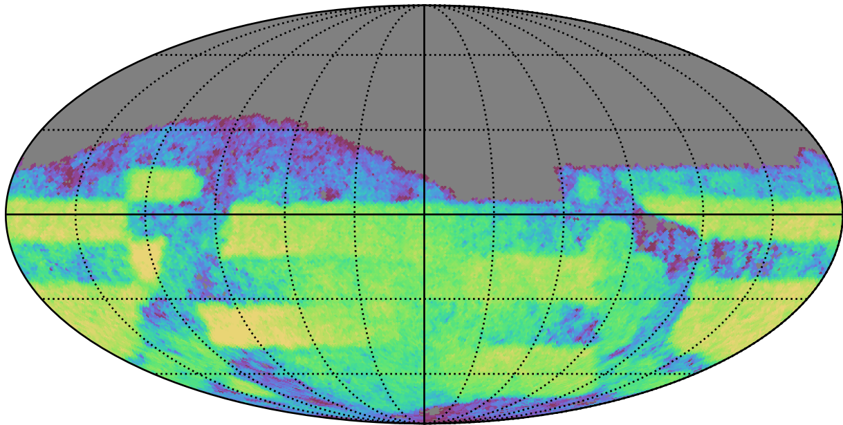
baseline_v3.2_10yrs Yr 3-4 z band: CoaddM5
