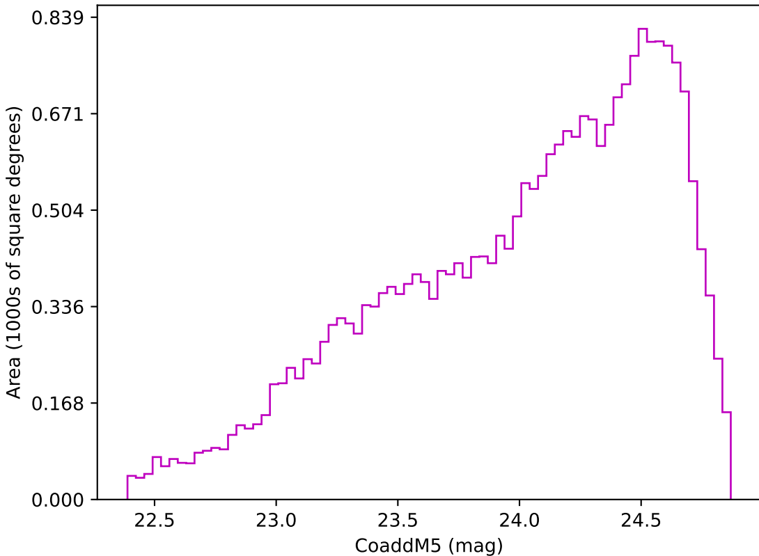
baseline_v3.2_10yrs Yr 3-4 z band: CoaddM5
