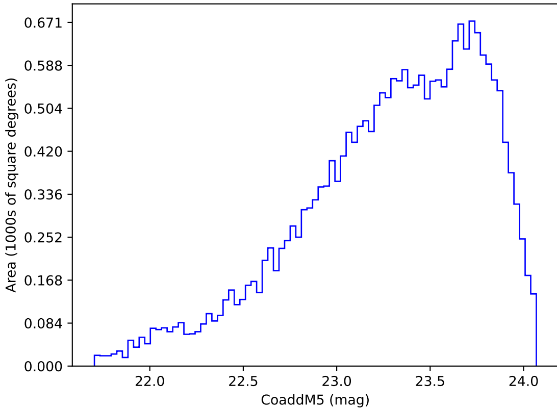
baseline_v3.2_10yrs Yr 3-4 y band: CoaddM5
