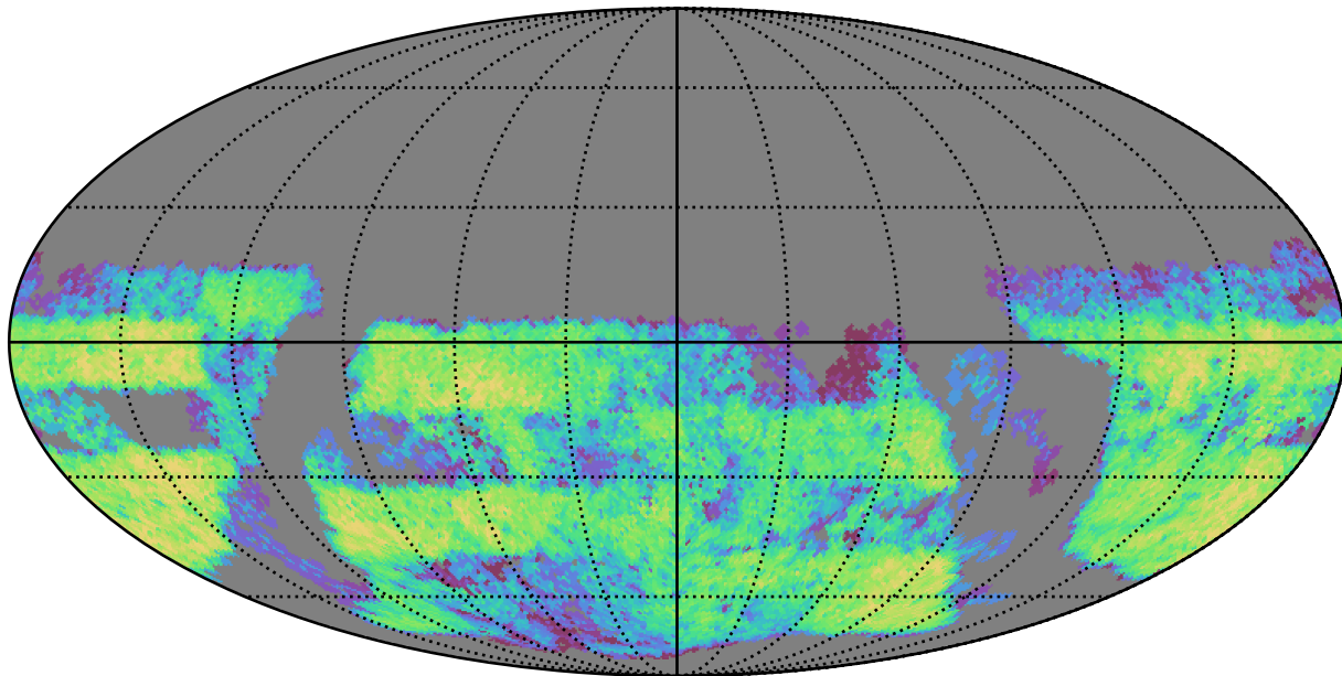
baseline_v3.2_10yrs Yr 3-4 u band: CoaddM5
