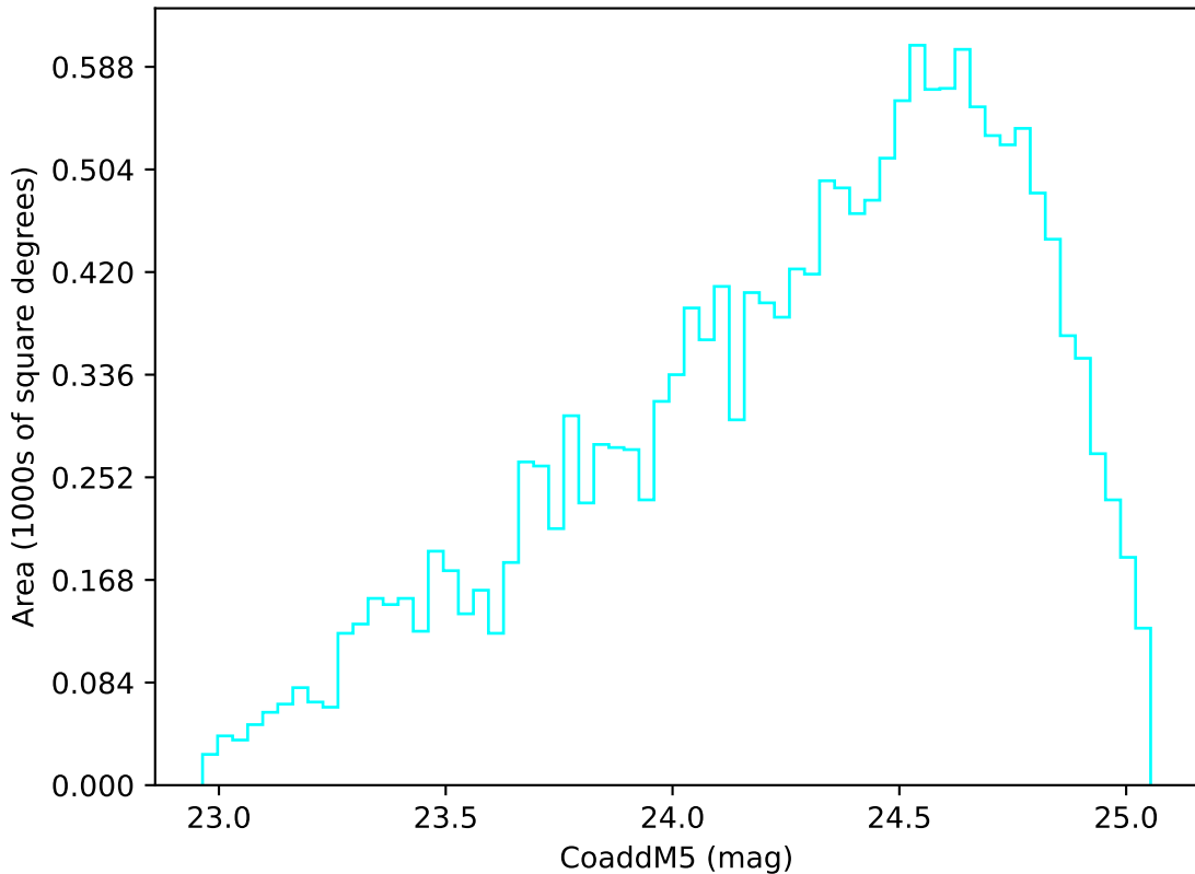
baseline_v3.2_10yrs Yr 3-4 u band: CoaddM5
