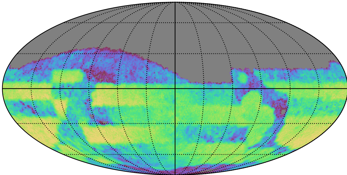
baseline_v3.2_10yrs Yr 3-4 r band: CoaddM5
