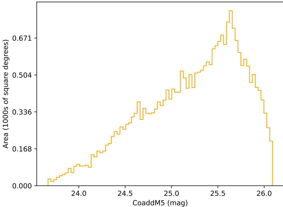
baseline_v3.2_10yrs Yr 3-4 r band: CoaddM5
