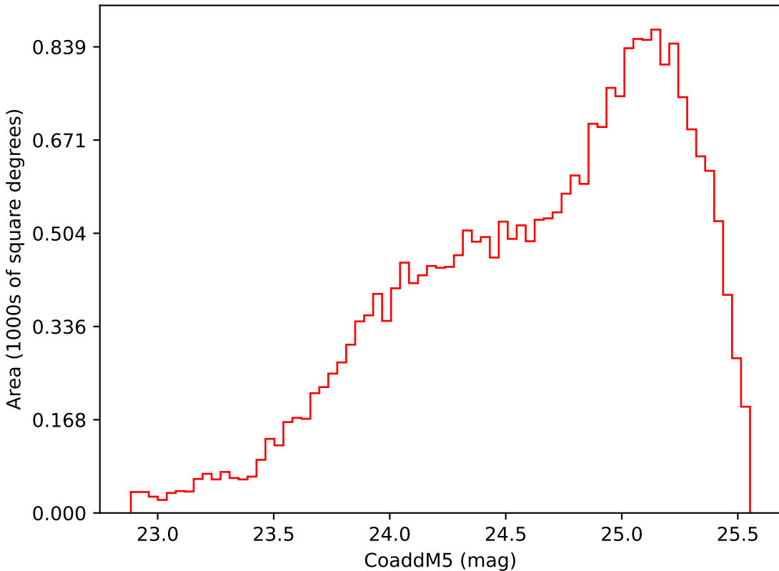
baseline_v3.2_10yrs Yr 3-4 i band: CoaddM5
