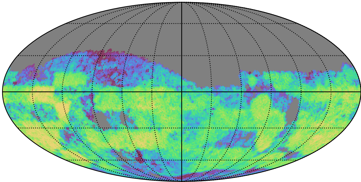
baseline_v3.2_10yrs Yr 3-4 g band: CoaddM5
