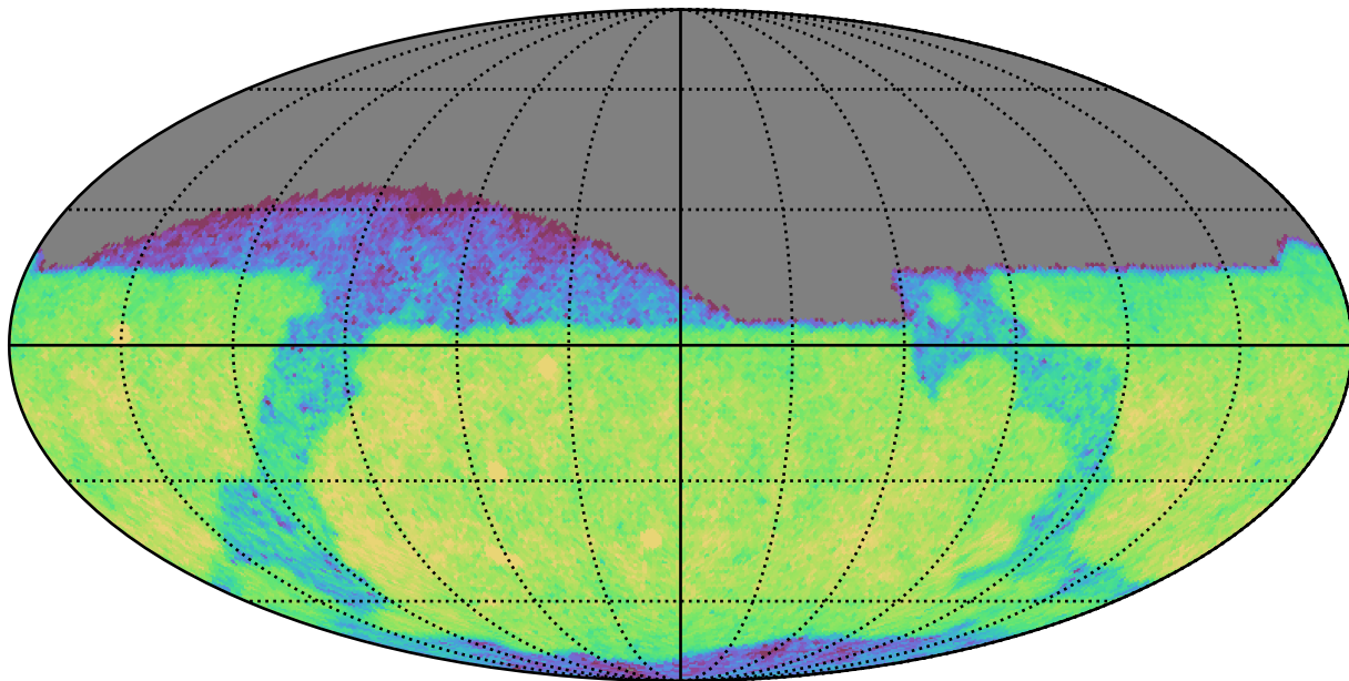
baseline_v3.2_10yrs Yr 1 z band: CoaddM5
