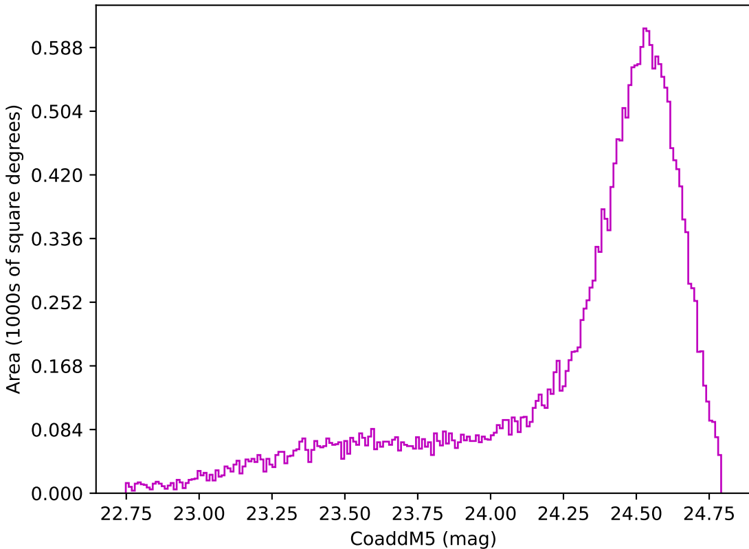
baseline_v3.2_10yrs Yr 1 z band: CoaddM5
