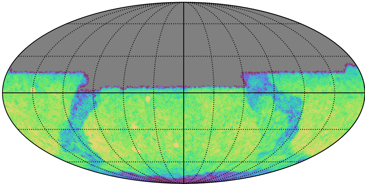
baseline_v3.2_10yrs Yr 1 y band: CoaddM5
