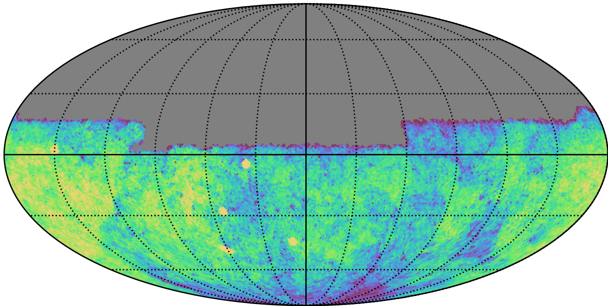
baseline_v3.2_10yrs Yr 1 u band: CoaddM5
