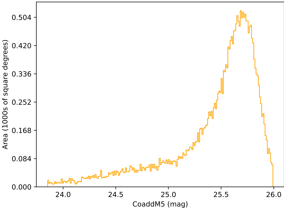
baseline_v3.2_10yrs Yr 1 r band: CoaddM5
