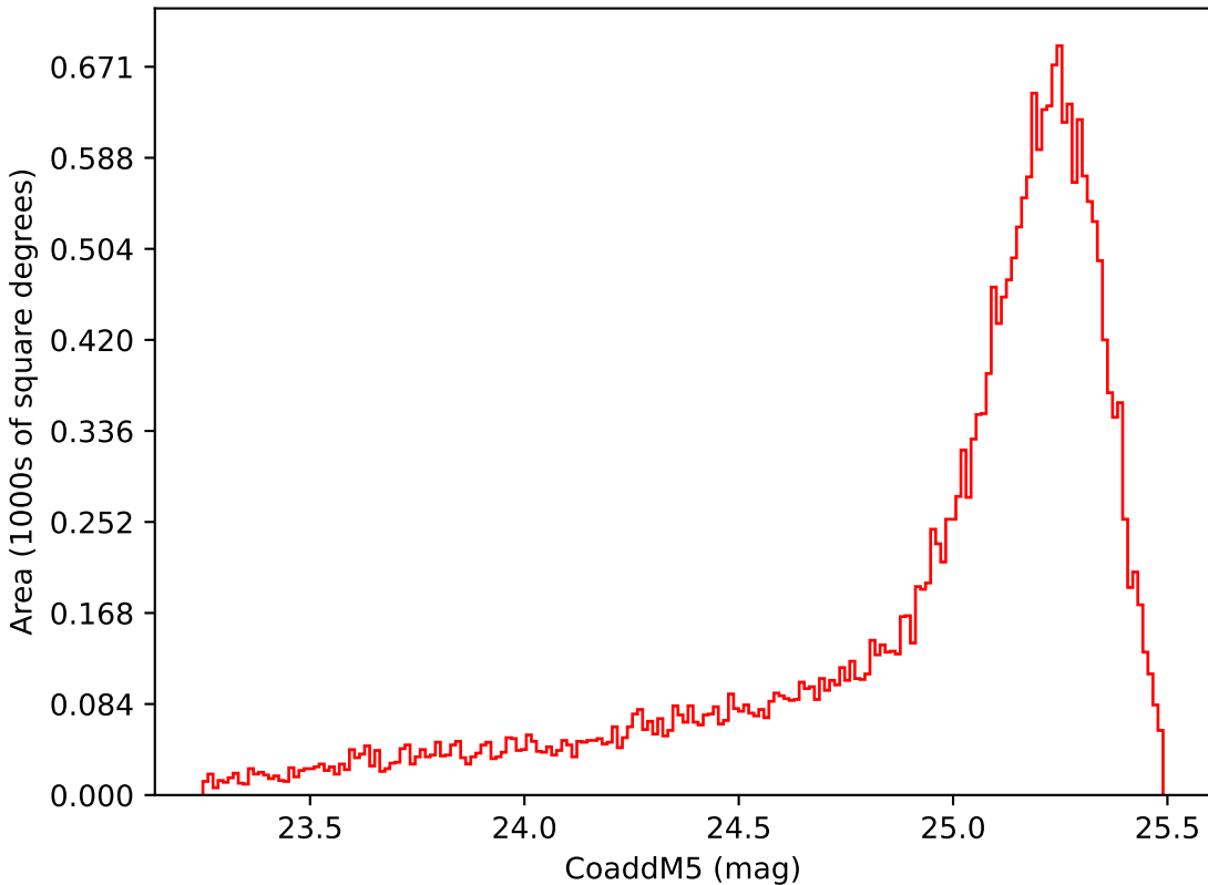
baseline_v3.2_10yrs Yr 1 i band: CoaddM5
