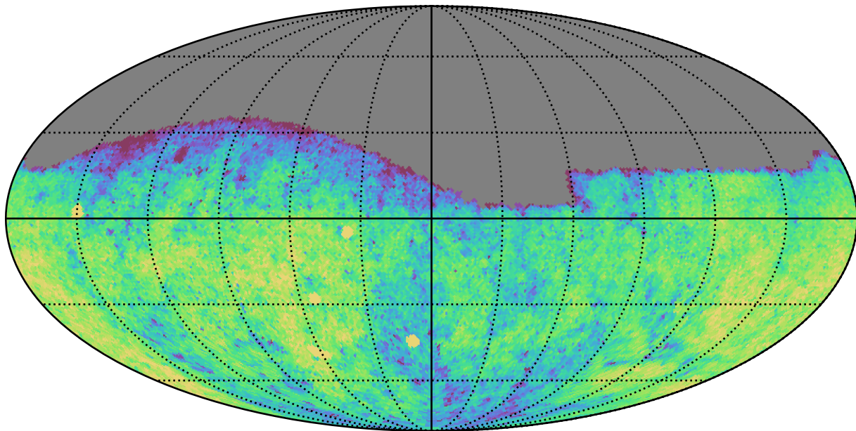
baseline_v3.2_10yrs Yr 1 g band: CoaddM5
