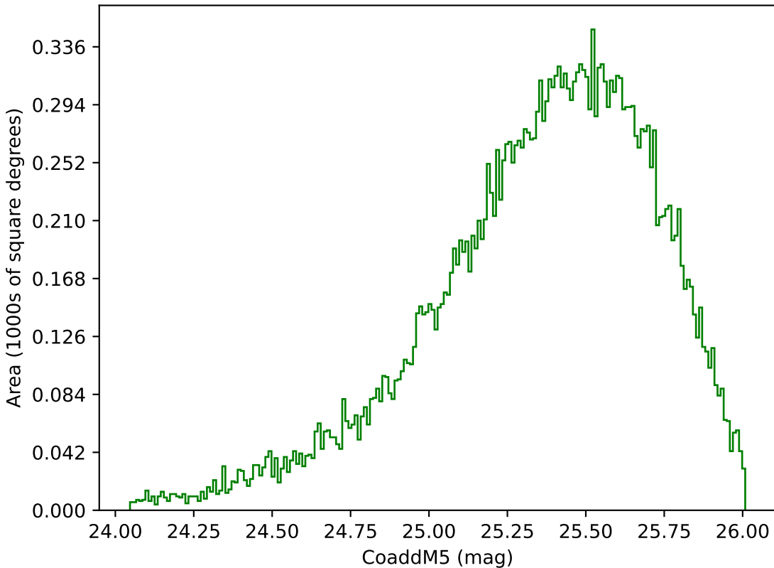
baseline_v3.2_10yrs Yr 1 g band: CoaddM5
