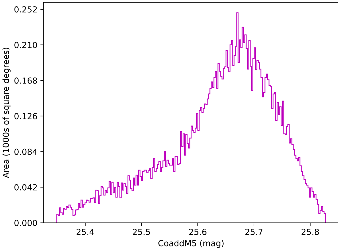
baseline_v3.2_10yrs WFD z band: CoaddM5
