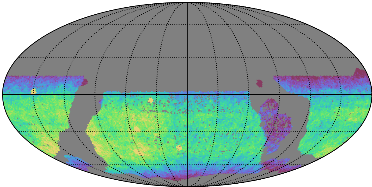
baseline_v3.2_10yrs WFD y band: CoaddM5
