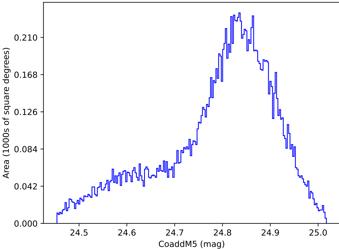
baseline_v3.2_10yrs WFD y band: CoaddM5
