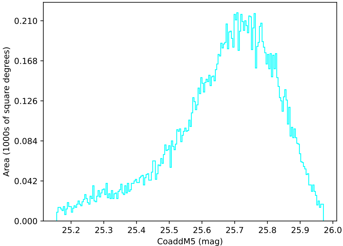
baseline_v3.2_10yrs WFD u band: CoaddM5
