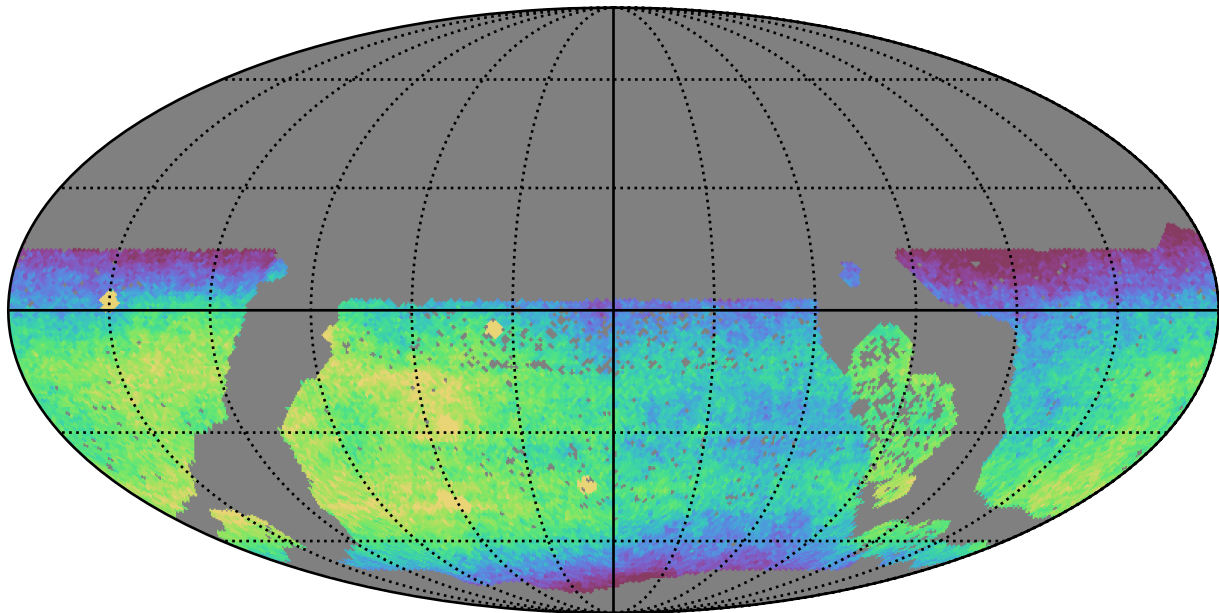
baseline_v3.2_10yrs WFD r band: CoaddM5
