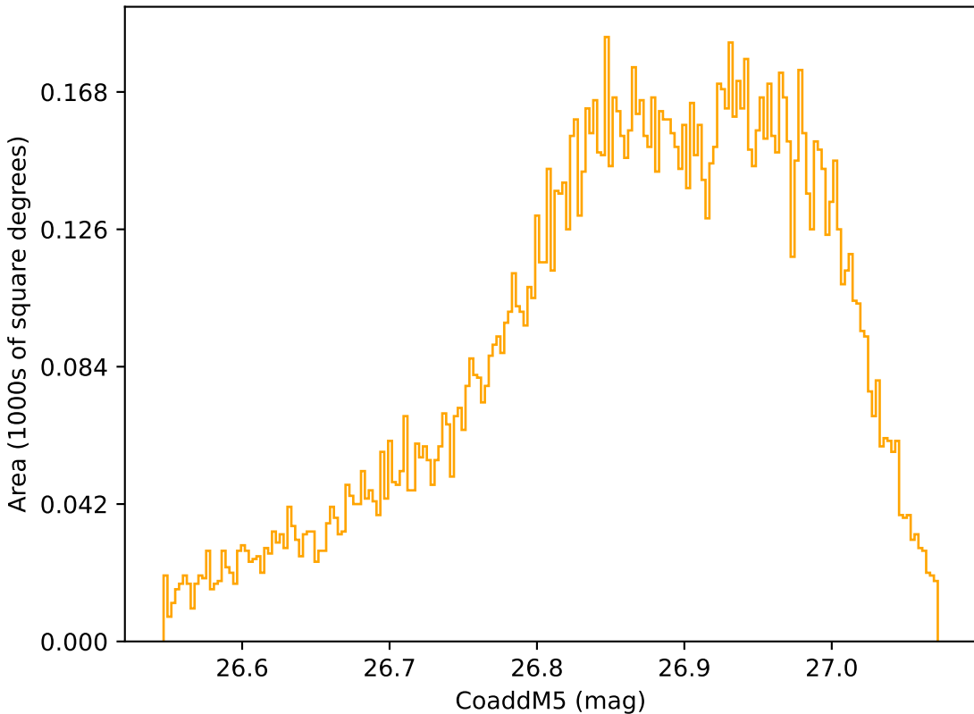
baseline_v3.2_10yrs WFD r band: CoaddM5
