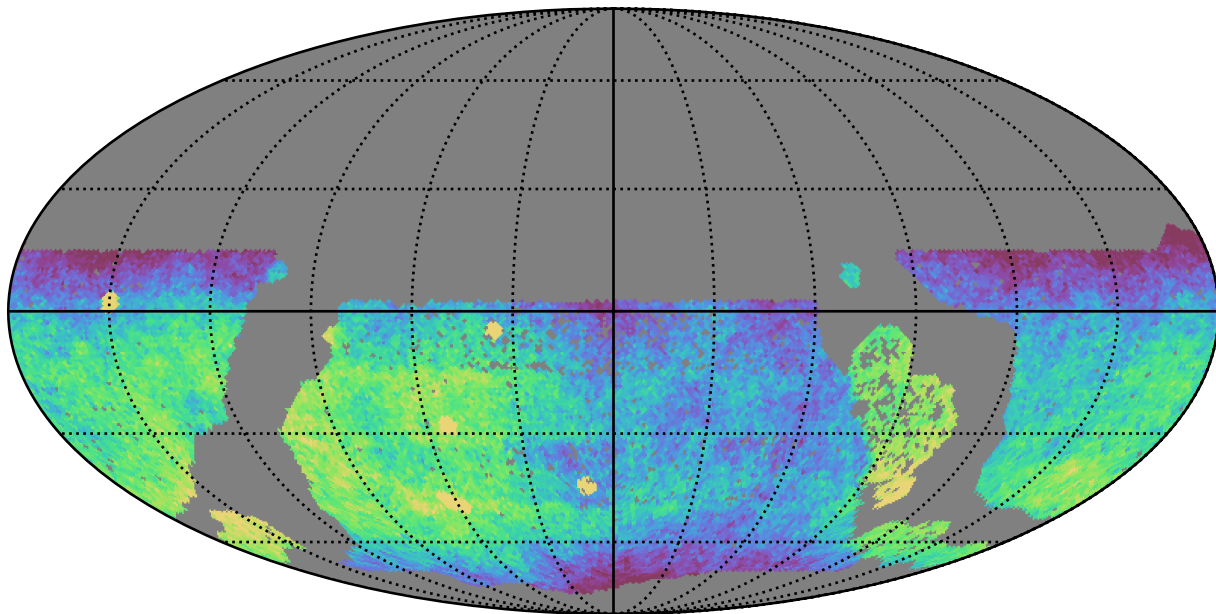
baseline_v3.2_10yrs WFD g band: CoaddM5
