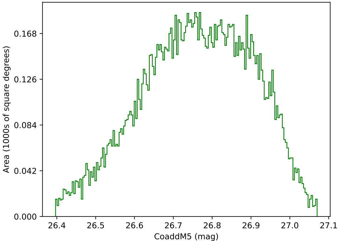
baseline_v3.2_10yrs WFD g band: CoaddM5
