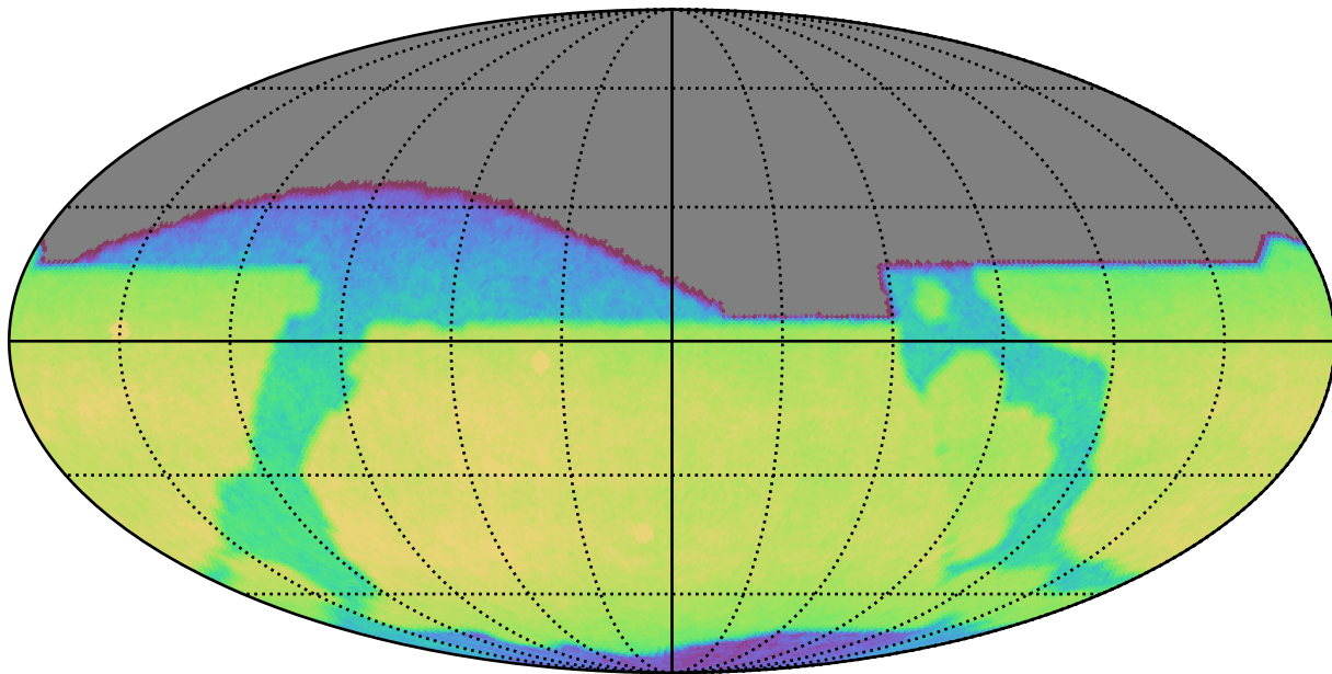
baseline_v3.2_10yrs All sky z band: CoaddM5
