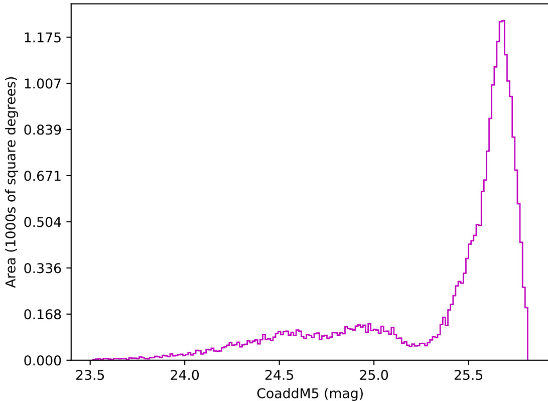
baseline_v3.2_10yrs All sky z band: CoaddM5
