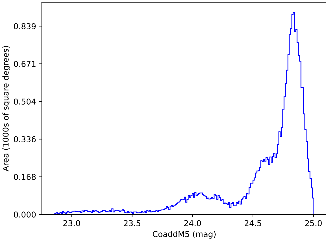
baseline_v3.2_10yrs All sky y band: CoaddM5
